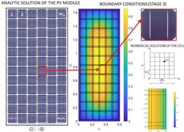
Fig. 3. Description of the numerical procedure: analytical evaluation of the boundary conditions (step #3) and numerical calculation of the temperature distribution inside the cell (step #4).
