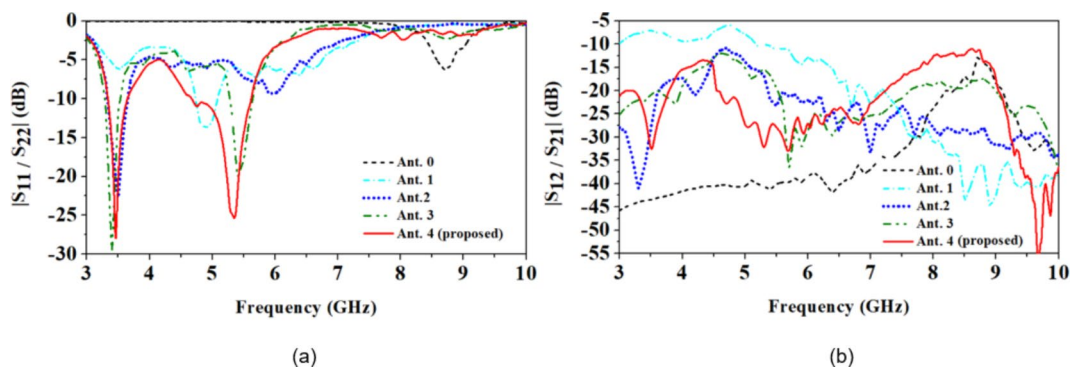
Fig. 6. S-parameters at each stage of the antenna evolution (a) S_{11}/S_{22} (b) S_{12}/S_{21} .
