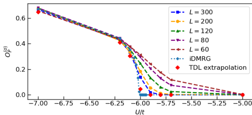
Figure 7: The figure shows the O_p^{(o)} results for: different sizes of a finite chain by DMRG, the thermodynamic limit extrapolation obtained by these sizes, and the same quantity obtained by the iDMRG method. The dashed and dotted lines are guide for the eyes.
