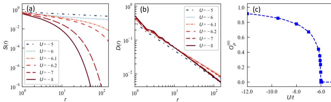
Figure 2: Analysis of a 1D system ( M = 1 ) at \bar{n} = 1 by performing iDMRG simulations with a maximum bond dimension of \chi_{\max} = 200 . The panels (a) and (b) present the analysis of the correlators in (2),(3) respectively. In the panel (c), the odd parity O_p^{(o)} is evaluated.
