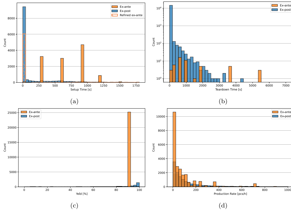
Fig. 4. Comparisons between ex-ante and ex-post distributions for the company numerical features.
