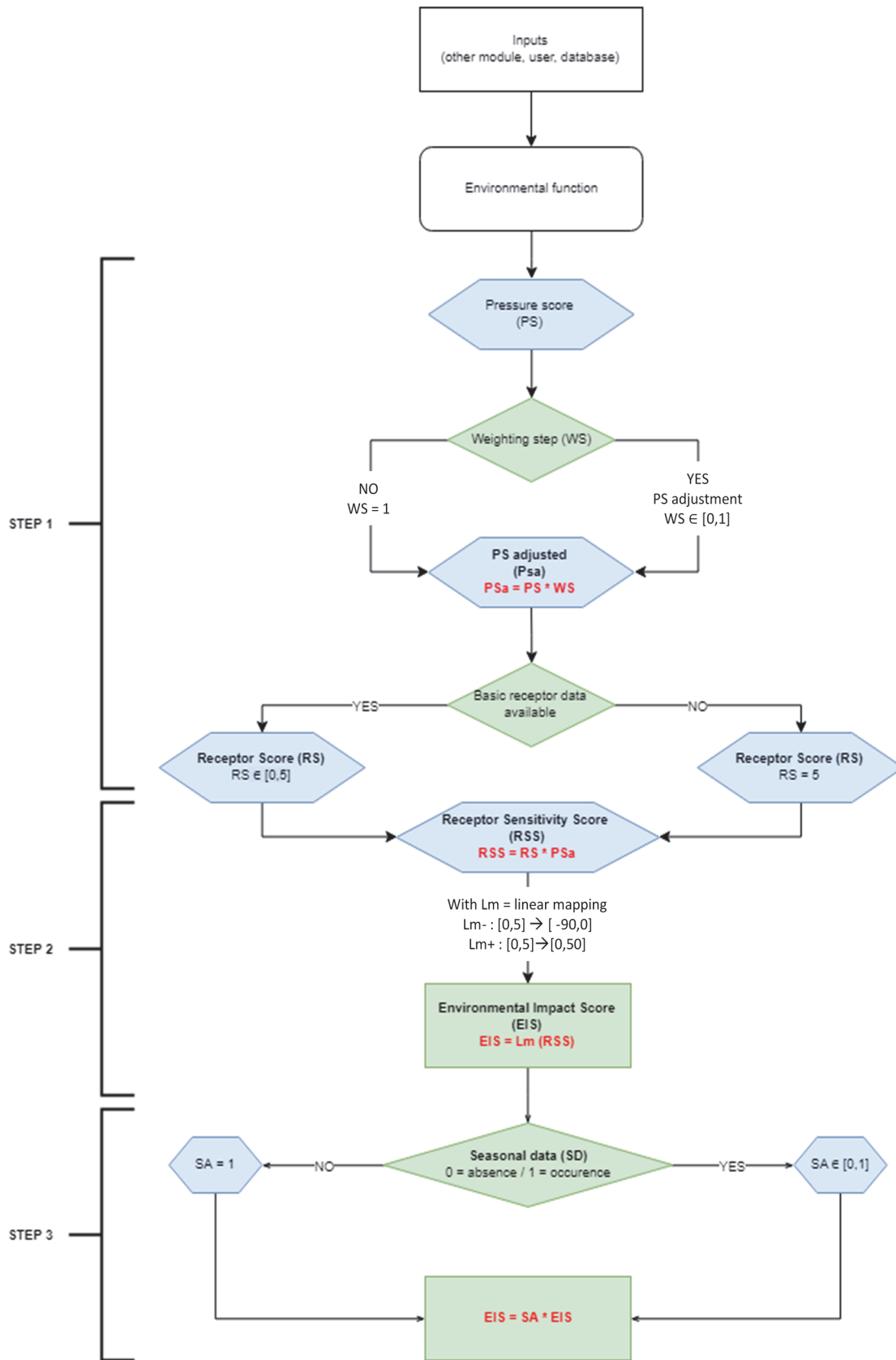
THREE-STEP SCORING ALGORITHM USED FOR EACH ENVIRONMENTAL PRESSURE IN THE ENVIRONMENTAL IMPACT ASSESSMENT FEATURE
