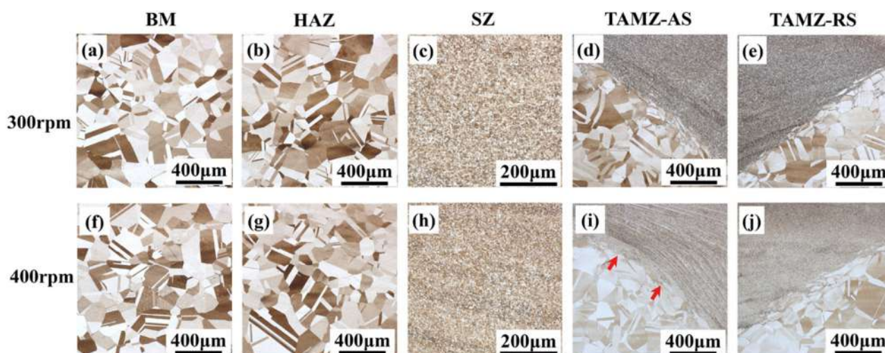
Figure 10. Butt FSW of 2.4 mm thick S32654. Optical images of various microstructural zones: BM (a,f), HAZ (b,g), SZ (c,h), TMAZ-AS (d,i) and TMAZ-RS (e,j) of 300 and 400 rpm, respectively ( v = 100 mm/min) [111]. Red arrows highlight the TMAZ region.
