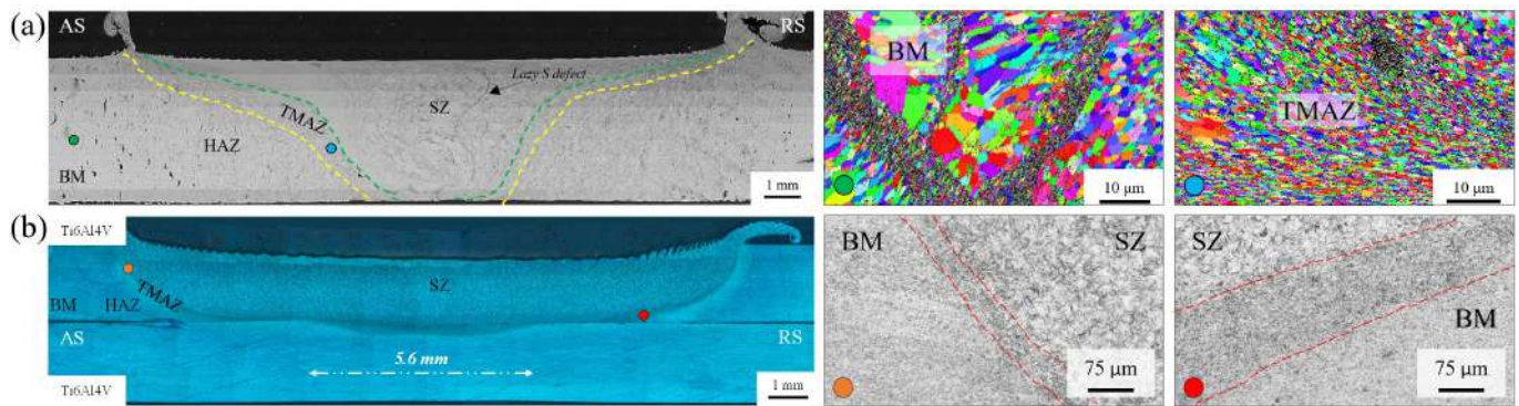
Figure 2. Examples of cross-section and typical regions of an FSW joint in (a) butt (Scalomalloy ® , 4 mm thick [4]) and (b) lap (Ti6Al4V, 2 mm thick [13]) configuration. Dotted lines highlight the boundaries between the joint areas (SZ, TMAZ, HAZ, and BM).
