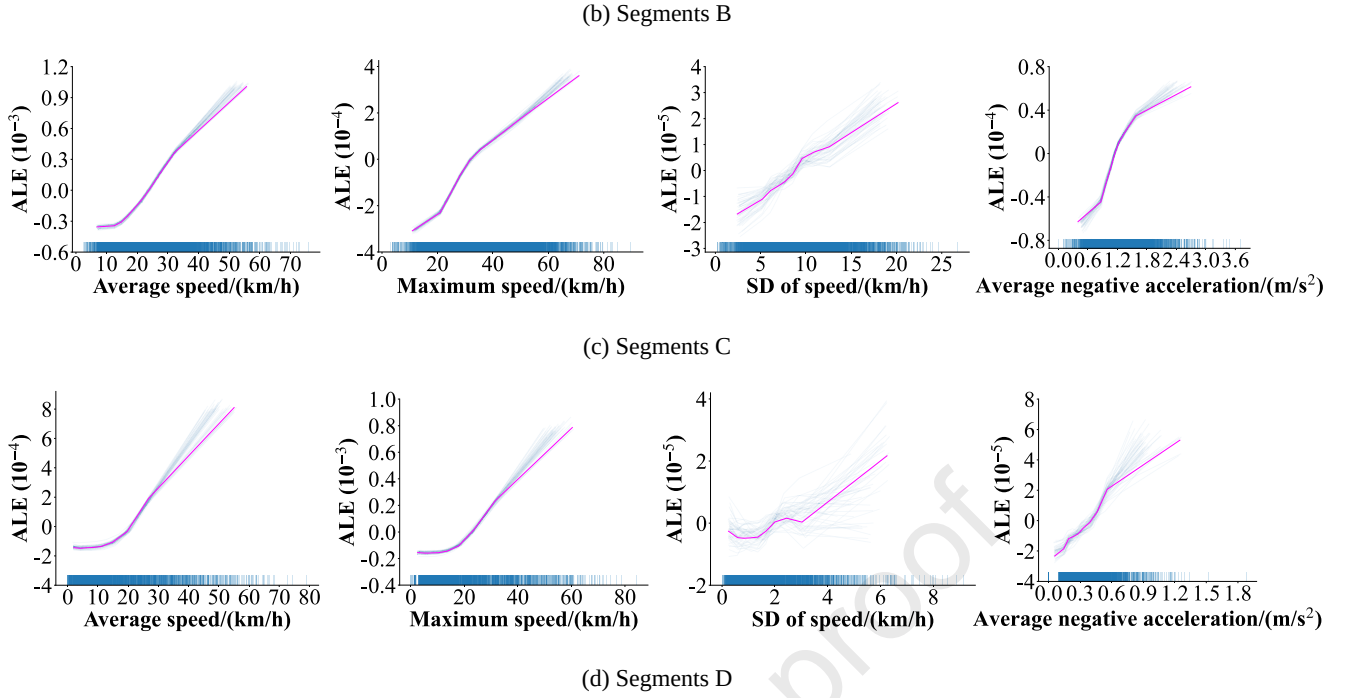
Fig. 8 ALE of important DBPs on VVCC
