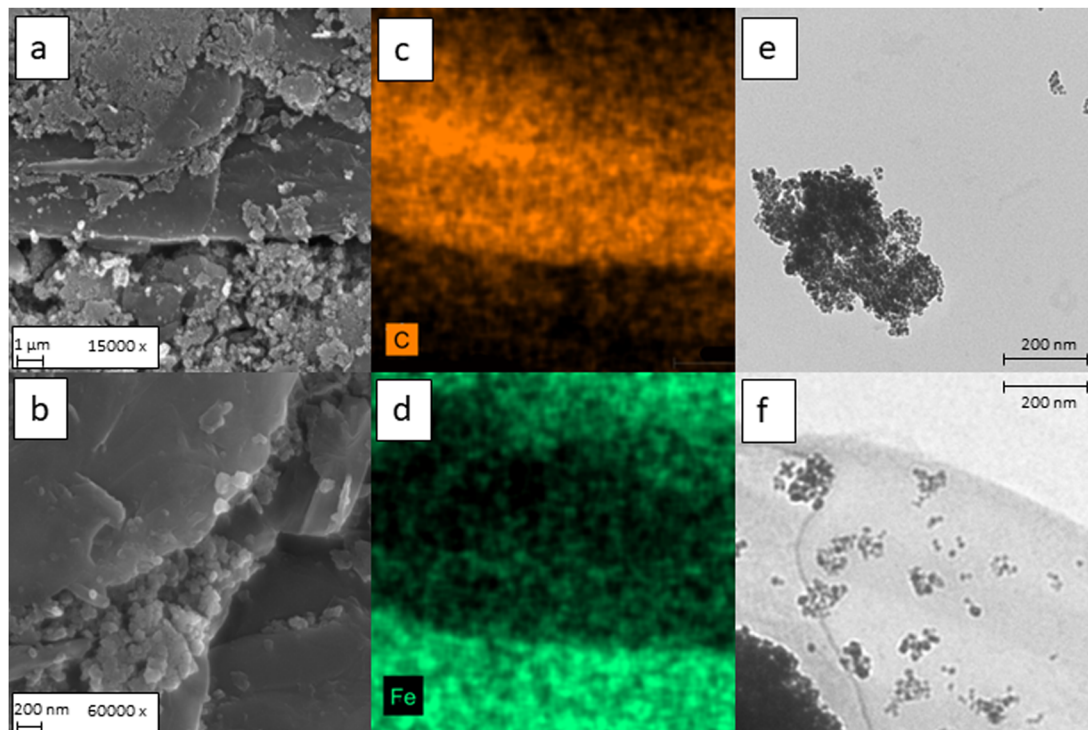
Fig. 3 SEM micrographs of \gamma - \text{Fe}_2\text{O}_3/\text{rGO} at (a) 15000x and (b) 60000x. EDS mapping at 15000x with highlighted (c) carbon and (d) iron. TEM micrographs of (e) bare \gamma - \text{Fe}_2\text{O}_3 and (f) \gamma - \text{Fe}_2\text{O}_3/\text{rGO} taken at 63000x.
