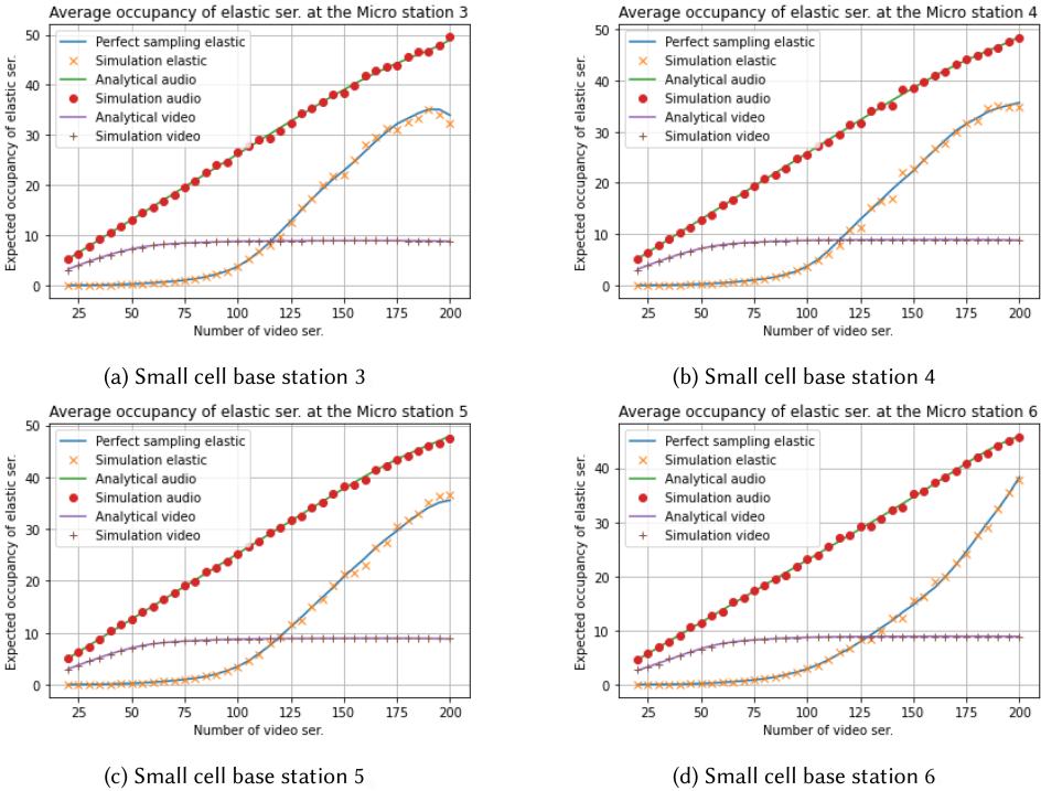
Fig. 10. Average number of streaming and elastic services active at each of the small cell BSs in the real BS layout.
