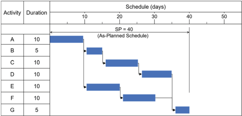
Figure 1. As-planned schedule of a sample project.
