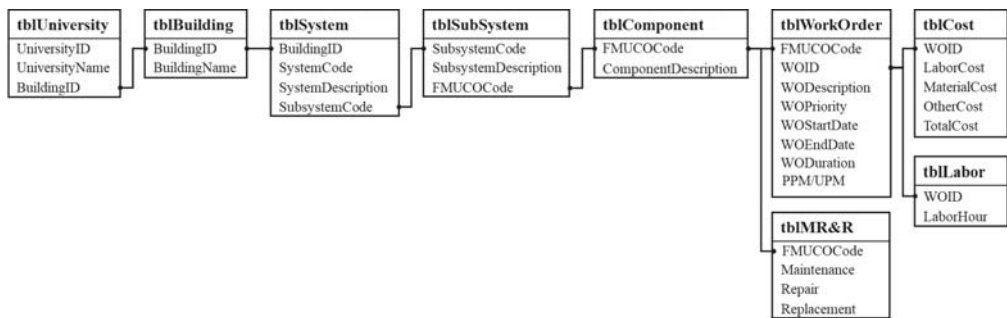
Figure 6. FMUCD structure.
