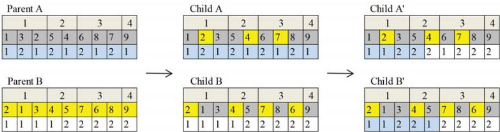
Figure 2. Schematic diagram of crossover operation.
