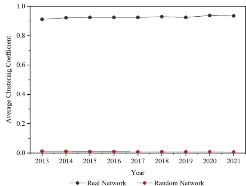
Figure 8. Change of the clustering coefficient of the collaborative networks in 2013–2021.
