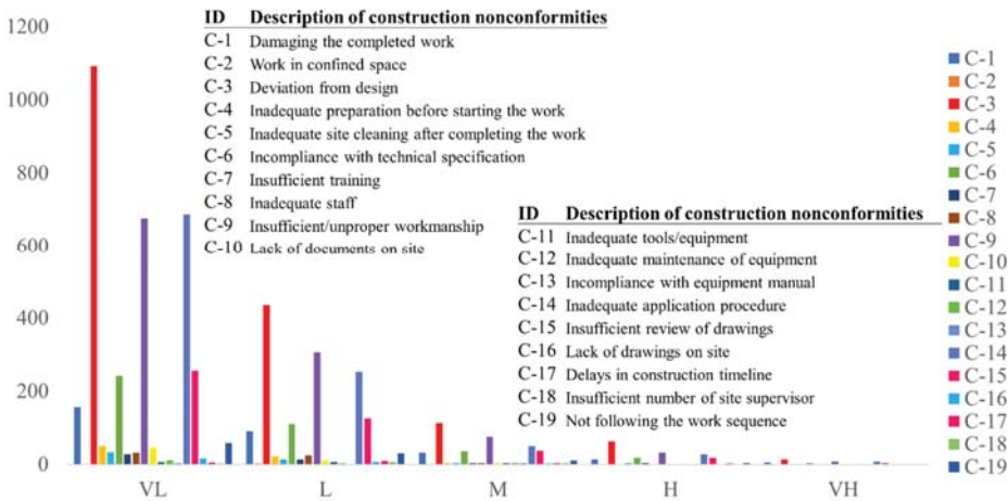
Figure 9. Construction-related nonconformance attributes.
