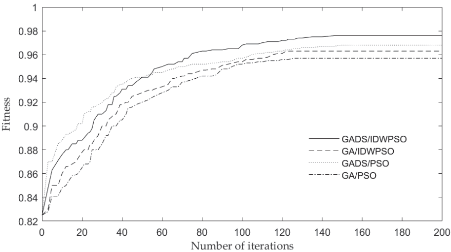
Figure 7. Algorithm iteration process.
