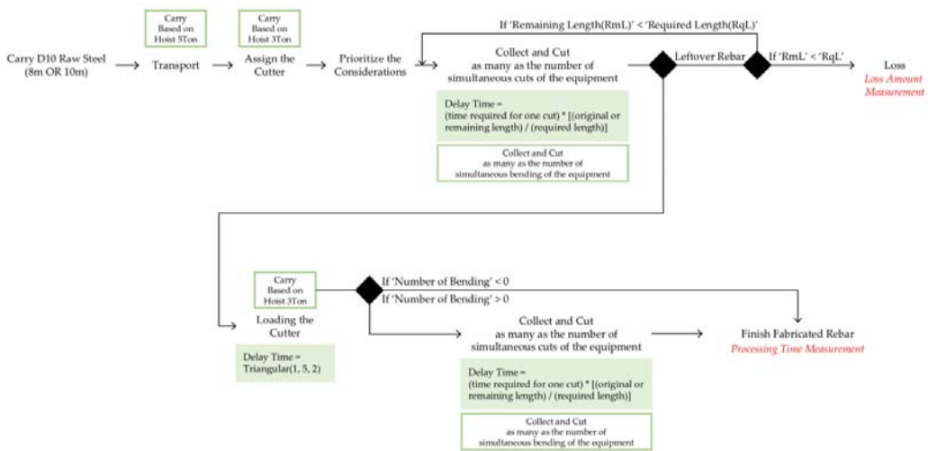
Figure 4. Simulation modeling that reflects processes within a rebar processing plant.
