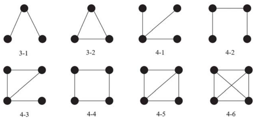
Figure 9. Topology of three-node and four-node subgroups.
