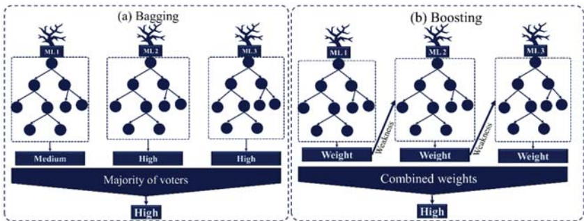
Figure 4. Simplified RF and boosting (AB and GB) ensemble mechanisms.
