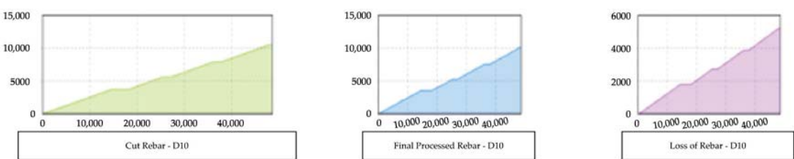
Figure 7. Model validation: D10 rebar time plot.
