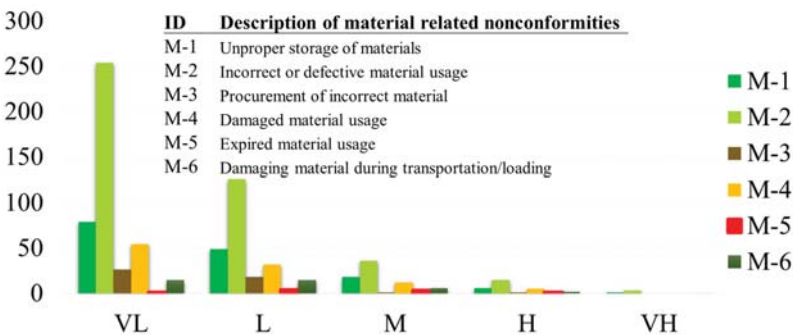
Figure 7. Material-related nonconformance attributes.
