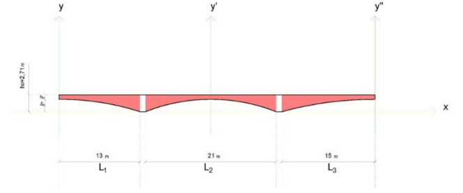
Fig. 3. Geometry of the main beam with non-constant section and reference axes
