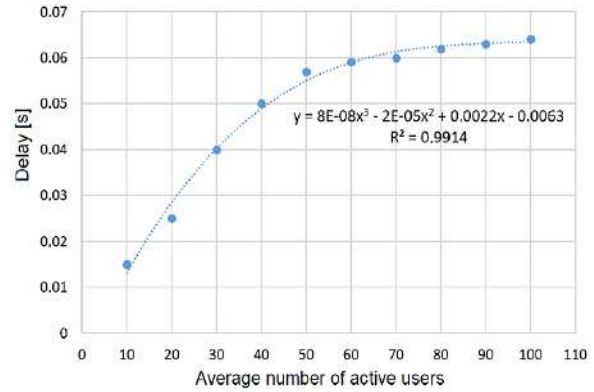
Fig. 3. Approximate cubic delay function
