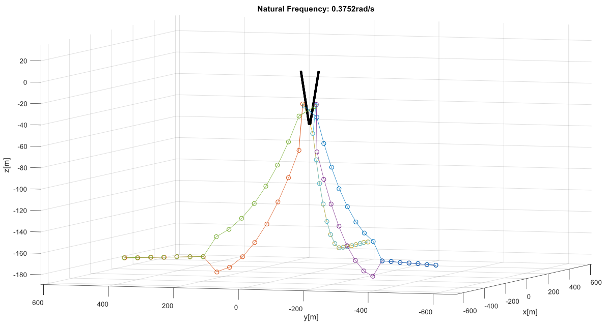
468 Figure 10. Modes of the coupled system mainly associated with pitch (top) and roll (bottom)
