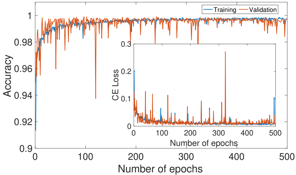
Figure 11: Accuracy and loss curves obtained using 2D-CNN on raw data, illustrating the model's performance without preprocessing.
