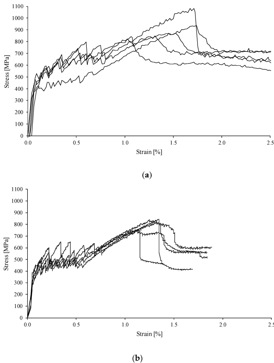
Figure 8. Stress–strain curves of tensile tests on series: (a) TT_T1; (b) TT_T2 (Data from [43]).
