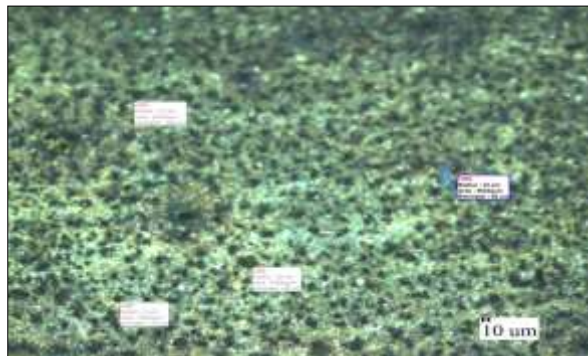
Fig. 10. Microstructure of oil tempered EN19 Steel Alloy (100x).
