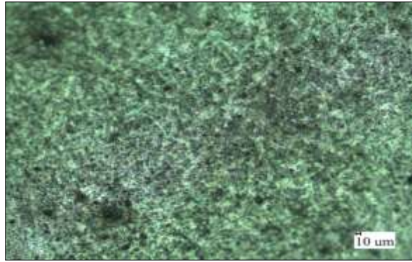
Fig. 6. Microstructure of brine quenched EN19 Steel Alloy (100x).
