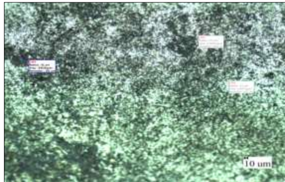
Fig. 3. Microstructure of normalized EN19 Steel Alloy (100x).
