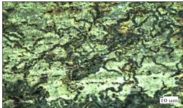
Fig. 4. Microstructure of annealed EN19 Steel Alloy (100x)
