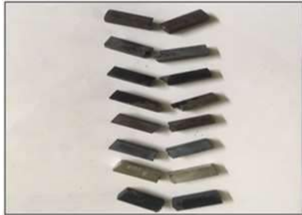
Fig. 13. Specimen after impact test.
