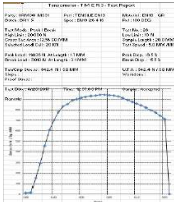
Fig. 11. Stress vs. strain graph for oil tempered specimen.
