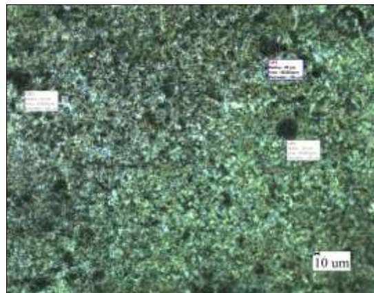
Fig. 2. Microstructure of untreated EN19 Steel Alloy (100x).
