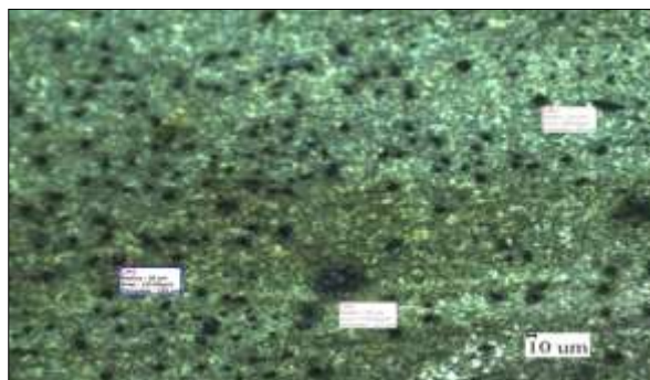
Fig. 5. Microstructure of water quenched EN19 Steel Alloy (100x).
