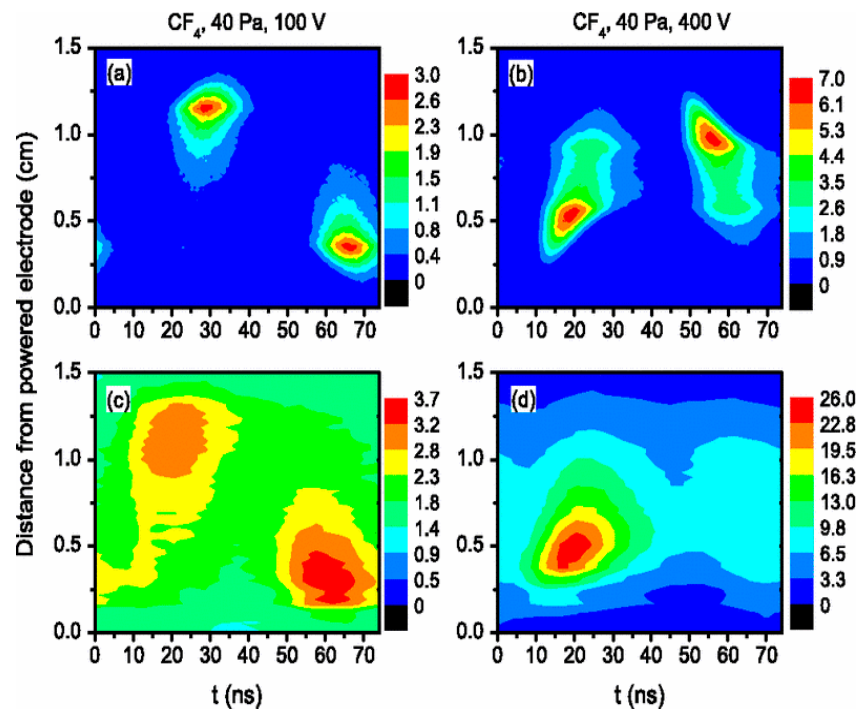
Figure 8. Plasma parameters as a function of time and space in a CF_4 discharge working at 40 Pa. In the first row, ionization rates from PIC-MCC simulations are reported in unit of 10^{21} \text{ m}^{-3} \text{ s}^{-1} for 100 V (a) and 400 V (b) peak bias voltages, while in the bottom row the measured plasma emission at 250 nm is reported in arbitrary units for 100 V (c) and 400 V (d) peak bias voltages. Reprinted with permission from [17]. Copyright (2011) by the American Physical Society.
