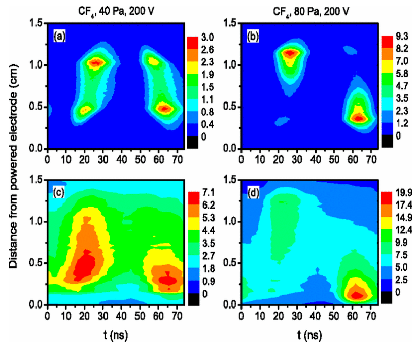
Figure 9. Plasma parameters as a function of time and space in a CF_4 discharge working at 200 V peak bias voltage. In the first row, ionization rates from PIC-MCC simulations are reported in units of 10^{21} \text{ m}^{-3} \text{ s}^{-1} for pressure of 40 Pa (a) and 80 Pa (b), while in the bottom row the measured plasma emission at 250 nm is reported in arbitrary units for pressure of 40 Pa (c) and 80 Pa (d). Reprinted with permission from [17]. Copyright (2011) by the American Physical Society.
