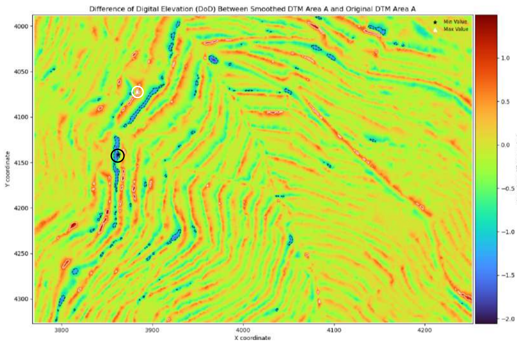
Fig.7: Difference of Digital Elevation of Area A
