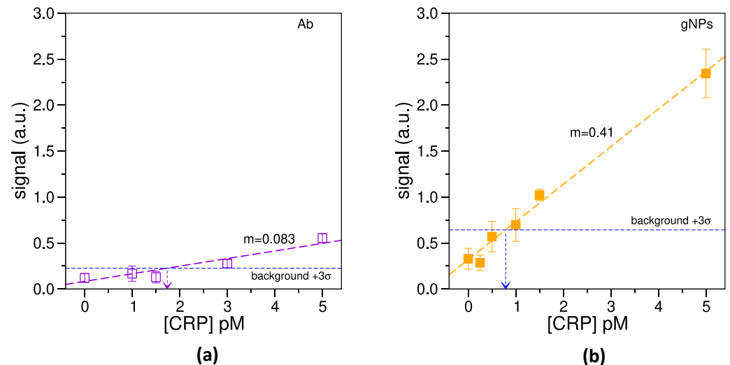
Figure 7. Estimation of LOD. (a): LOD measured for LFT performed with pure a-CRP-HRP; (b): LOD measured for LFT with the functionalized gNPs.
