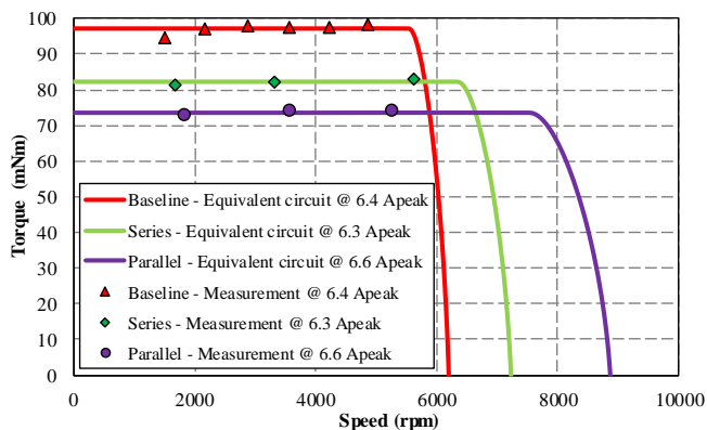
Fig. 17: Torque-speed measurements for three prototyped machines.
