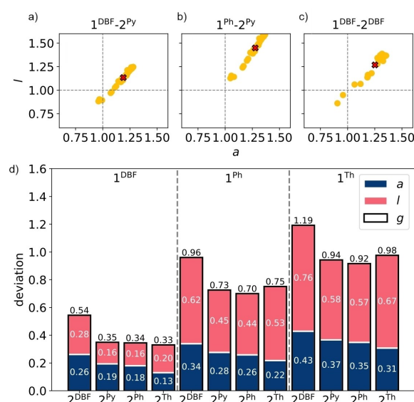
Figure 6. Plots of angle ( a ) and length ( l ) deviations for conformer libraries of a) \text{1}^{\text{DBF}} and \text{2}^{\text{Py}} , b) \text{1}^{\text{Ph}} and \text{2}^{\text{Py}} , and c) \text{1}^{\text{DBF}} and \text{2}^{\text{DBF}} . Red crosses denote average a and l values. d) Charts of average deviation values for all ligand combinations.
