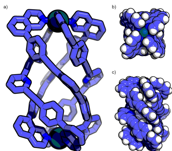
Figure 3. SCXRD structure of the \Lambda enantiomer of [Pd 2 (2 Py ) 4 ] 4+ a) from the side, with hydrogen atoms omitted for clarity, and space-fill models shown b) down the Pd–Pd axis, and c) from the side.
