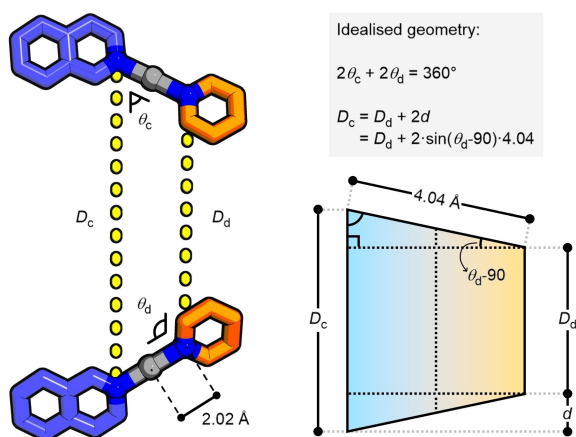
Figure 5. Cartoon representation of the coordination angles within an idealised heteroleptic \text{cis-Pd}_2\text{L}_2\text{L}'_2 assembly.
