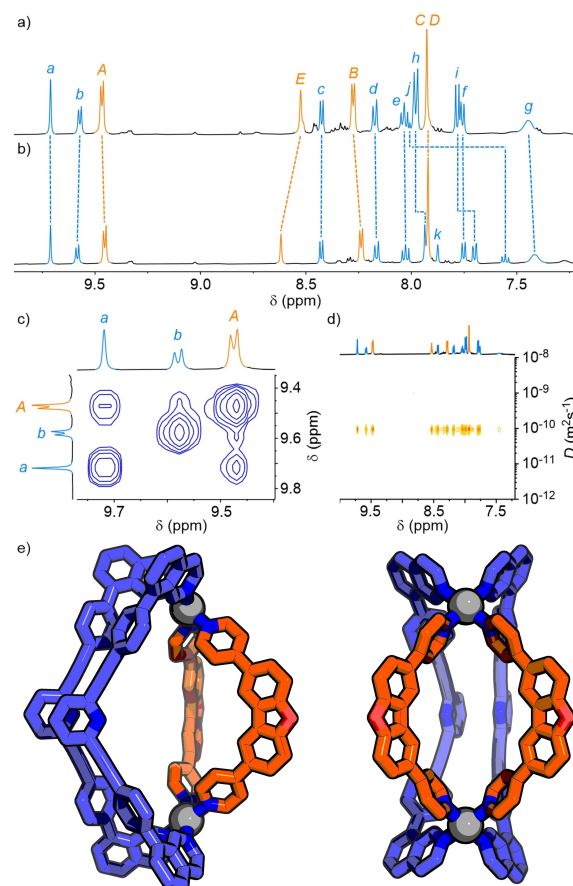
Figure 4. 1 H NMR spectra (500 MHz, d 6 -DMSO, 298 K) of a) [Pd 2 (1 DBF ) 2 (2 Py ) 2 ](BF 4 ) 4 and b) [Pd 2 (1 DBF ) 2 (2 Ph ) 2 ](BF 4 ) 4 ; c) partial NOESY of [Pd 2 (1 DBF ) 2 (2 Py ) 2 ](BF 4 ) 4 showing interactions between ligands 1 DBF and 2 Py , and d) DOSY of [Pd 2 (1 DBF ) 2 (2 Py ) 2 ](BF 4 ) 4 . e) DFT-optimised structure (PBE0/Def2-SVP/D3BJ/PCM(DMSO)) of cis -Pd 2 (1 DBF ) 2 (2 Py ) 2 ] 4+ .
