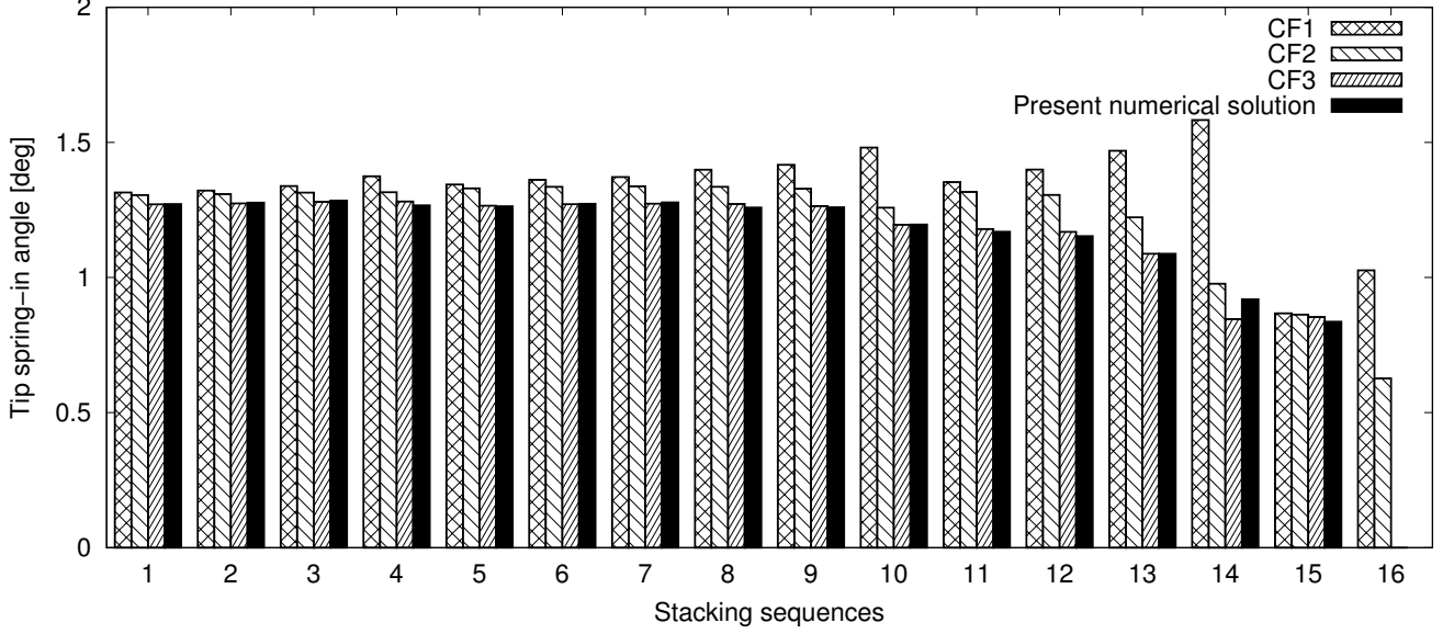
Figure 12: Comparison of tip spring-angles for symmetric stacking sequences from analytical and numerical simulations. For stacking sequence 16: CF1 = 1.0265^\circ , CF2 = 0.6264^\circ , CF3 = 0.0^\circ , Present numerical solution = -4.9054E-05^\circ .
