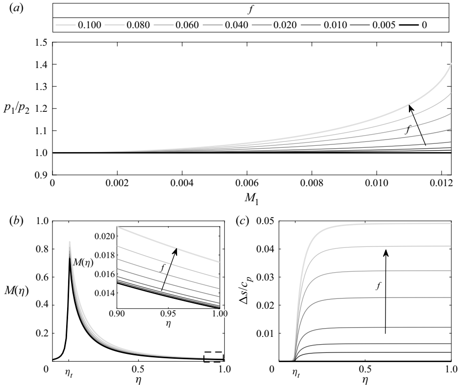
Figure 3. Mean flow: (a) ratio of inlet and exit pressures, (b) Mach number and (c) entropy. The arrows indicate increasing friction, f . The normalised throat location is \eta_t = 0.095 .
