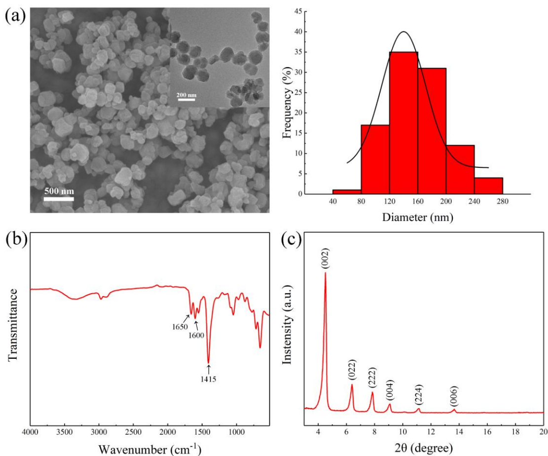
Fig. 1. (a) Morphology images and diameter distribution of the synthesized MOF. (b) FTIR spectrum of MOF. (c) XRD patterns of MOF.
