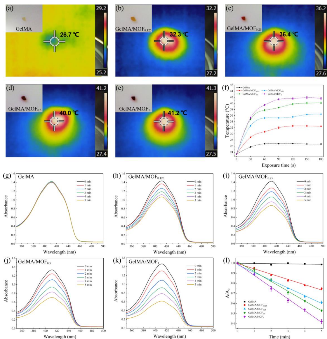
Fig. 6. (a-e) Digital images and surface thermal under visible illumination ( \sim 30 mW/cm 2 ) for 180 s. (f) Temperature rise curves. (g-k) UV-vis spectra of DPBF under
