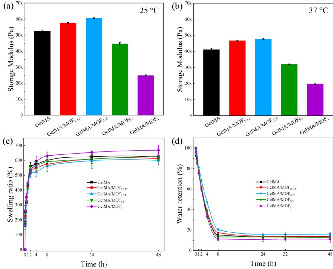
Fig. 5. (a-b) Storage modulus of 3D-printed GelMA and GelMA/MOF hydrogels at 25 °C and 37 °C, respectively. (c) Swelling ratio. (d) Water retention.
