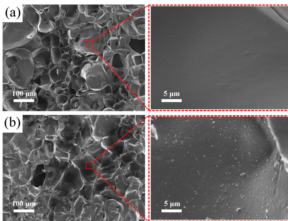
Fig. 4. Morphological structures of 3D-printed GelMA (a) and GelMA/MOF 1 hydrogels (b).
