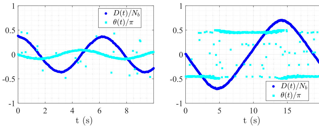
FIG. 3. Examples for the dynamical evolution of the conjugate variables D and \theta for a trajectory in the Josephson oscillations region (left) and for a trajectory in the \pi oscillations region (right). The trajectories belong to the phase portrait in Fig. 2.
