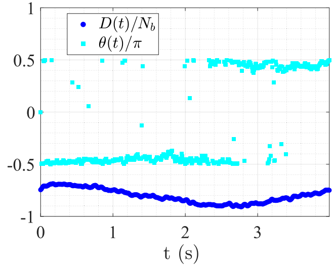
FIG. 7. Time evolution of D and \theta for a self-trapped trajectory of the phase portrait in Fig. 6. In this example, the trajectory is the highly nonlinear regime, in the island-like region: both variables feature small oscillations around a nonzero average.
