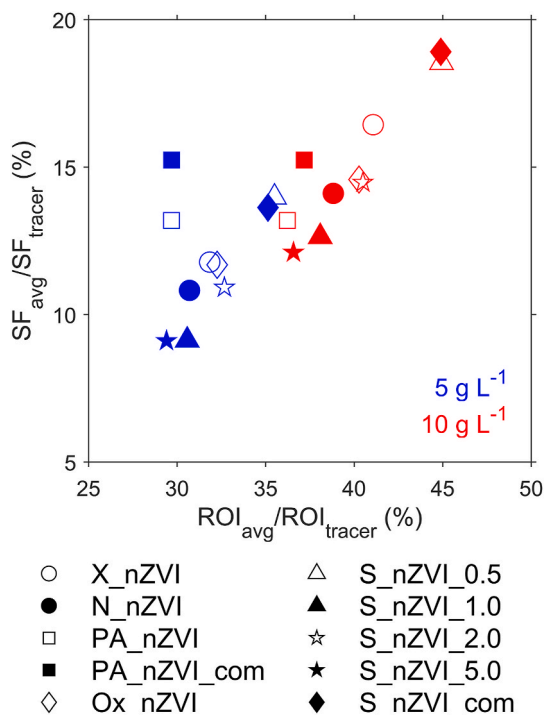
Fig. 5. Normalization of ROI and SF against non-interacting tracer for enhanced comparability of X_nZVI and its derivatives transport.
