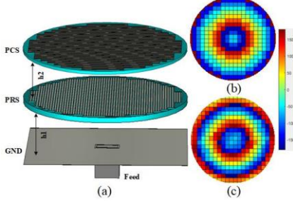
Figure 2. (a) The designed PRS antenna; (b) The compensation phase distribution from Formula (1); (c) The compensation phase distribution from Ansys HFSS.
