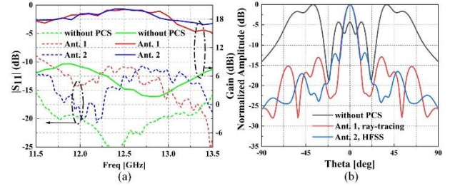
Figure 4. Simulation results for PRS antennas without PCS and with the PCS designed by the proposed ray-tracing method or Ansys HFSS: (a) Realized gain and |S_{11}| ; (b) Radiation patterns.
