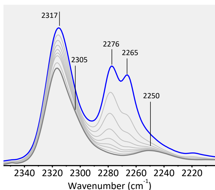
Figure 4. Evolution of the FT-IR spectra, in the \tilde{\nu}(\text{C}\equiv\text{N}) region, for \text{CD}_3\text{CN} adsorbed at room temperature on Cr(VI)/ \text{SiO}_2 +TEAL(2:1) catalyst as a function of the \text{CD}_3\text{CN} coverage (blue: maximum coverage, dark grey: irreversible fraction of \text{CD}_3\text{CN} , light grey: intermediate coverages).
