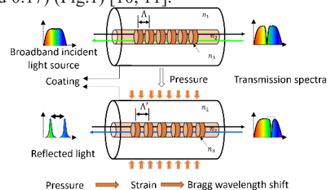
Fig.1. Transduction mechanism: elastomeric-coated FBG pressure sensing ( n_1 's - refractive indices and \Lambda - grating length) The longitudinal strain sensitivity and lateral pressure sensitivity of FBG are given by equations (1) and (2) [9].
