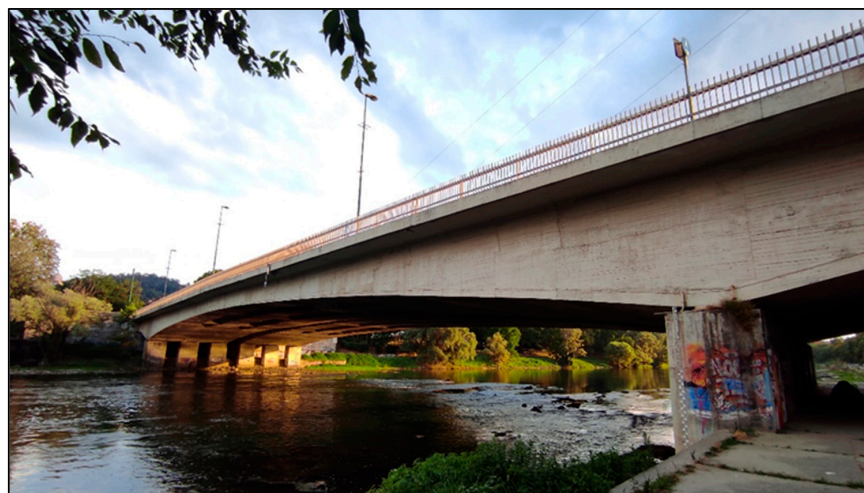
Figure 8. Close-up view of the Corso Regina Margherita Bridge (V1-T), which is the subject of this and other ongoing research.
