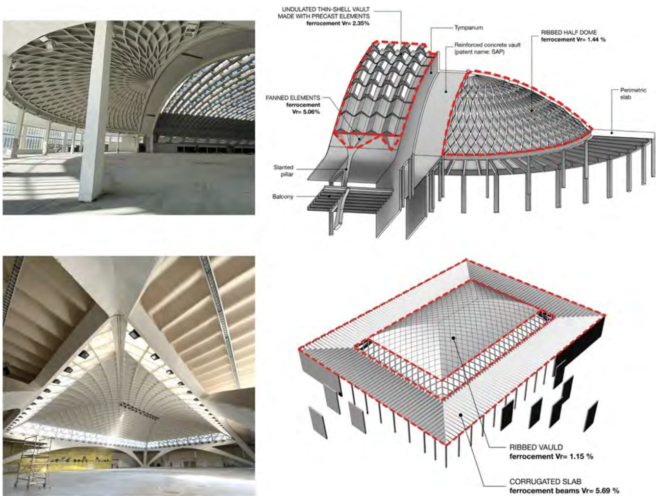
FIGURE 1 Interior view of Nervi's halls in Torino Esposizioni and their schematization showing where the main ferroement elements are located and their volumetric steel fraction in percentage. On the top is reported the Hall B, while the Hall C is on the bottom.
