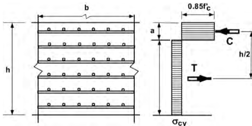
FIGURE 6 Plastic moment method. 8
