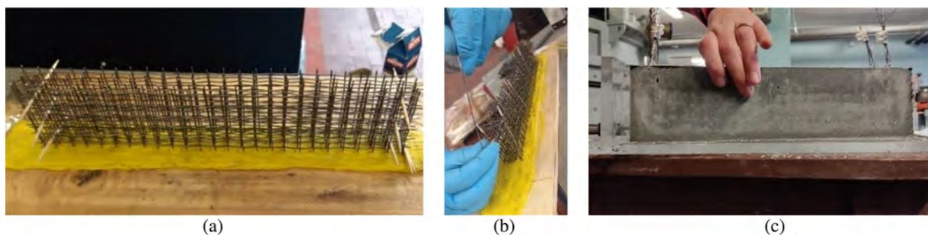
FIGURE 5 Ferrocement samples realization (a) net layers positioning (b) steel connections for subsequent corrosion potential measure (c) casted sample.
