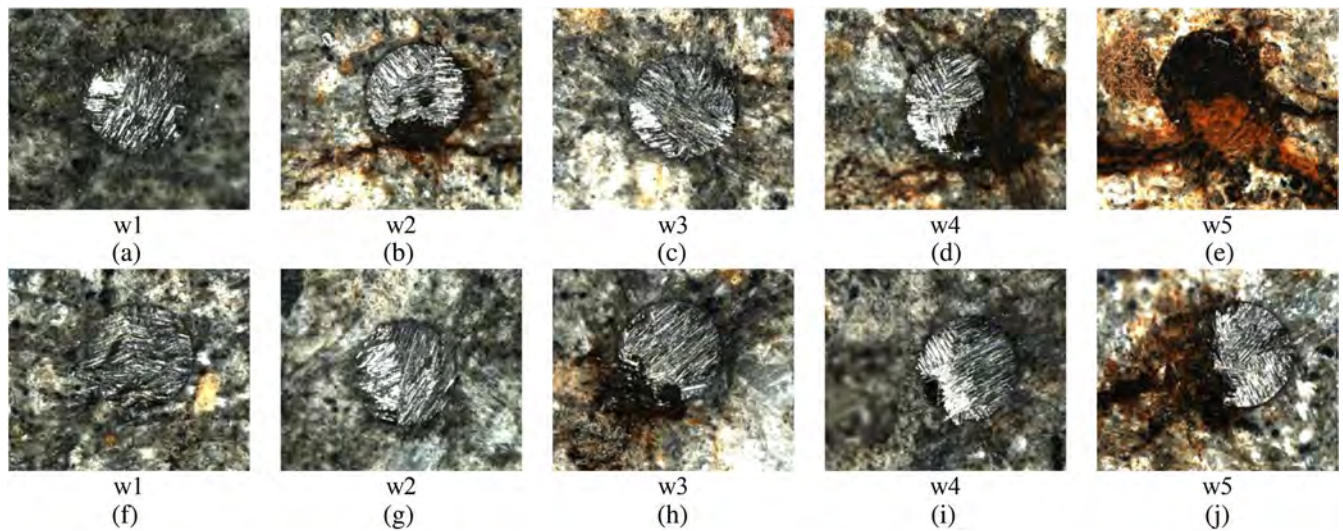
FIGURE 17 Photographic acquisitions of the corrosion state of wires of sample Aged_02 (a–e) and the painted and aged sample (f–j), by means of the optical microscope (magnification 5\times ).
