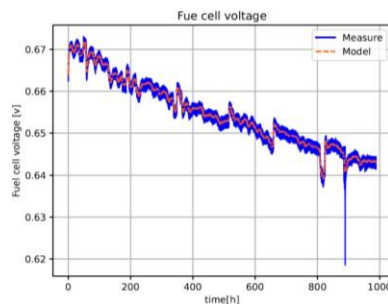
Fig. 2: Fuel Cell Voltage Model
