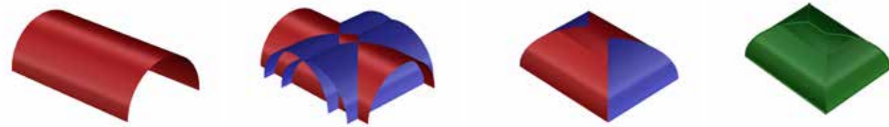
3b 1.4. (above): an internal view of the space of Hall C. (below) A classic geometric generation of a barrel vault with pavilion heads
