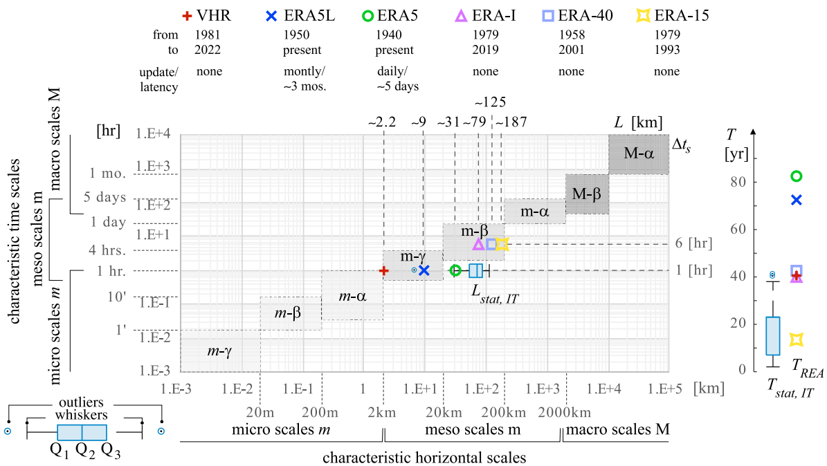
Fig. 3. Space and time scales of the atmospheric processes, synopsis of the time series duration T , horizontal resolution L and sampling period \Delta t_s of the reanalysis models [REA, specifically ERA-15, ERA-40, ERA-Interim (ERA-I), ERA5, ERA5-Land (ERA5L), VHR-REA_IT (VHR)], and of the Italian land anemometric stations used in Ballio et al. (1999) to draw the Italian wind map (DM 17-01-2018).
