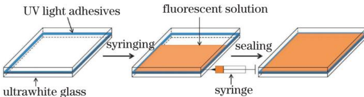
Fig. 1. Schematic of fabricating process of the aqueous layer LSC device.
