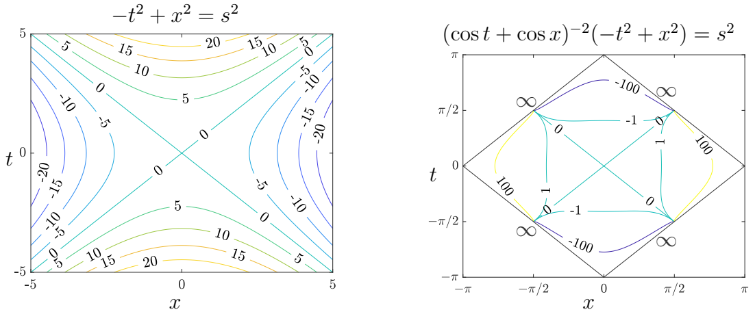
(a) Minkowski space in classic coordinates.
