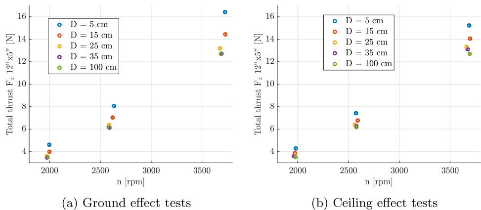
Fig. 14 Relationship between motor speed and total thrust of the UAV in and out of ground and ceiling effects for 12'' \times 5'' propellers
