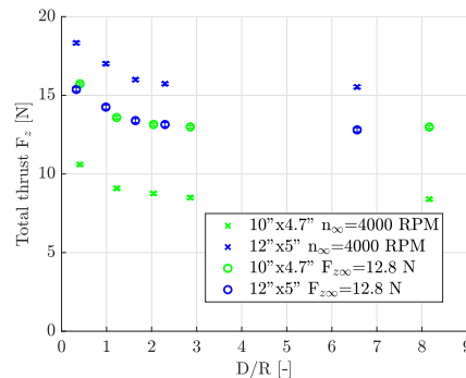
(b) Results at PWM levels between 1600 \mu s and 2000 \mu s for 10”x4.7” (green markers) and 12”x5” (blue markers) propellers
