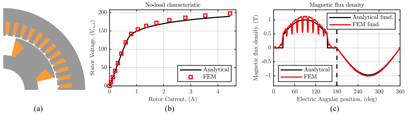
Fig. 9. Results for WFSM1: 2D sketch (a), no-load characteristic (b), air gap flux density (c).
