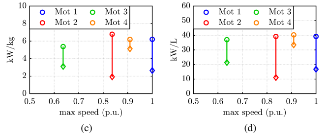
Fig. 6. Torque and power densities function of the maximum motor speed. Circle refers to peak condition and diamonds refers to max speed condition
