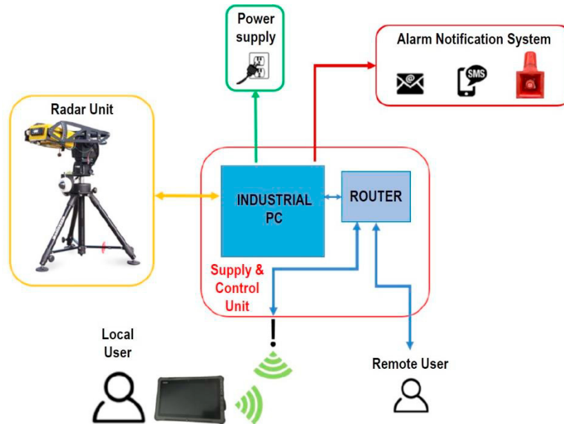
Fig. 5. Schematic outline of an EWS based on GB-InSAR monitoring to be applied to major tunnel rehabilitation works.
