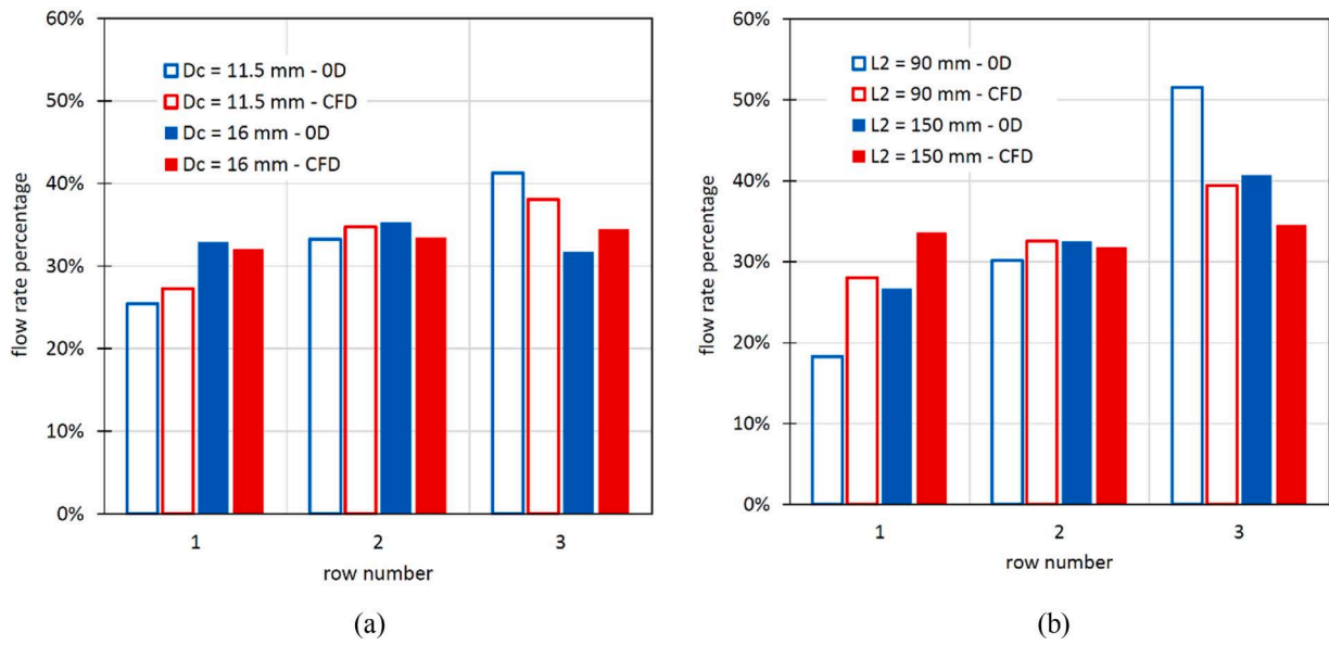
Fig. 22. Comparison between the CFD and the OD model with variable coefficients and stationary shaft: (a) variation of the diameter of the axial channel, (b) variation of the distance between the rows.
