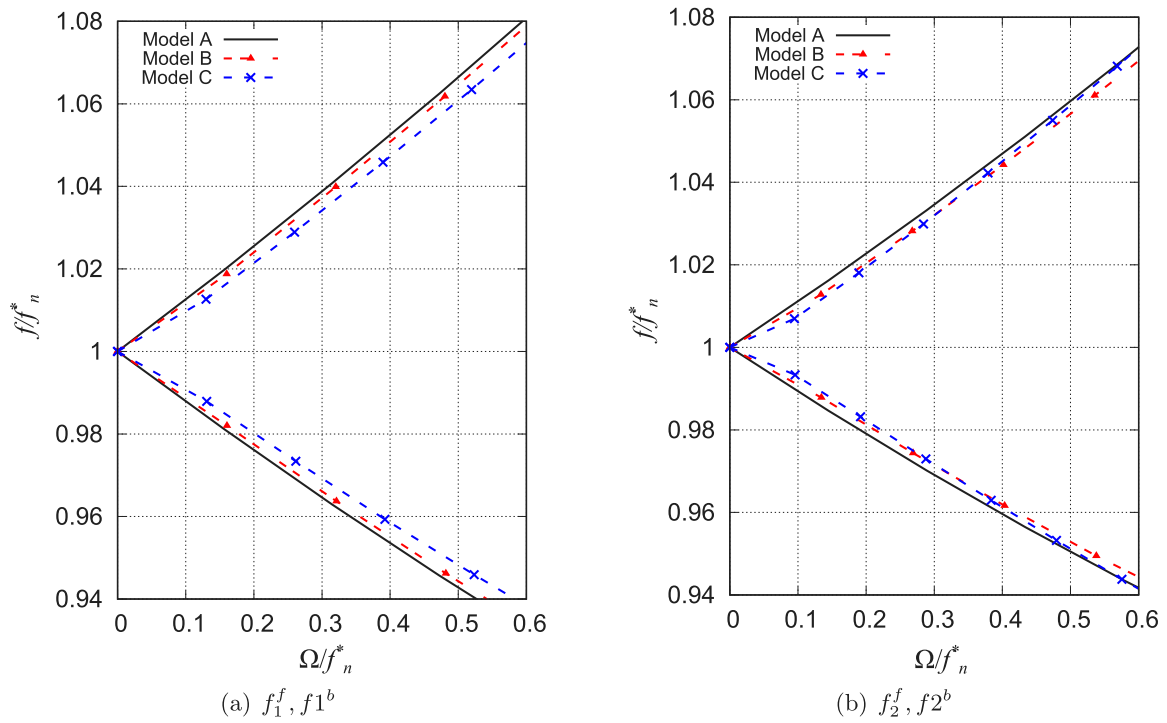
Fig. 15. Campbell diagrams of the free-free thick cylinder with: Model A = [90^\circ/0^\circ/90^\circ] ; Model B = [90^\circ + (0^\circ/30^\circ)/0^\circ + (0^\circ/30^\circ)/90^\circ + (0^\circ/30^\circ)] ; Model C = [90^\circ + (75^\circ/30^\circ)/0^\circ + (75^\circ/30^\circ)/90^\circ + (75^\circ/30^\circ)] . f_n^* indicates the value of the associated frequency at \Omega = 0 rad/s.
