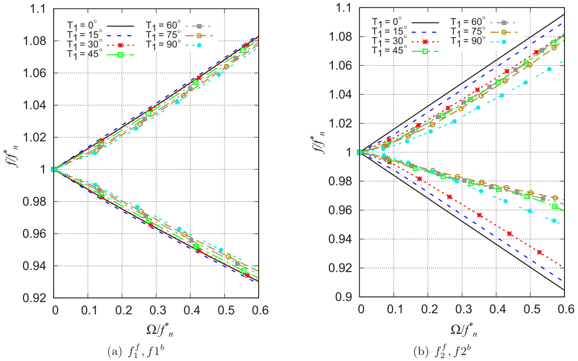
Fig. 12. Effect of T_1 on the Campbell diagram of the first two vibration modes. Thin cylinder with \theta = [90^\circ + (0^\circ/T_1)/0^\circ + (0^\circ/T_1)]_s . f_n^* indicates the value of the considered frequency at \Omega = 0 rad/s.
