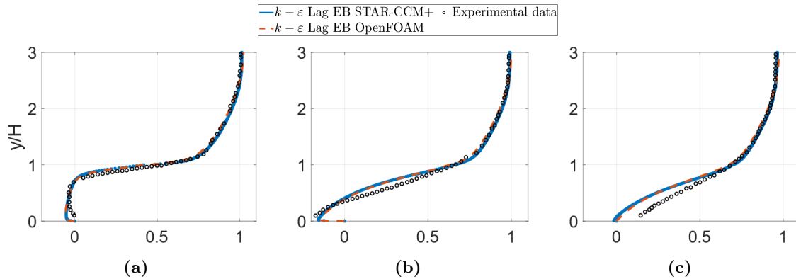
Figure 4. Normalized velocity magnitude, U/U_{ref} : (a) x/H = 1 , (b) x/H = 4 , (c) x/H = 6
