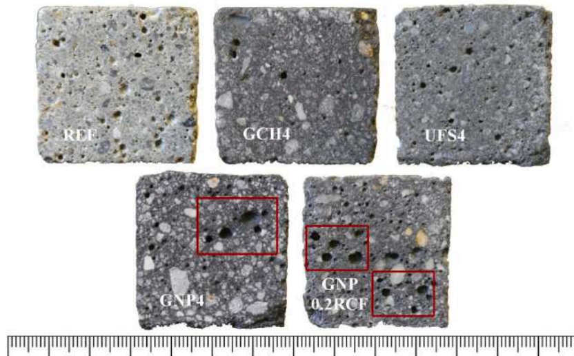
Fig. 10. Comparison of the internal section of different mortar mixes with voids highlighted in red in GNP mortars (the scale is in mm). (For interpretation of the references to colour in this figure legend, the reader is referred to the Web version of this article.)
