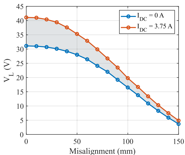
FIGURE 16. Variation of V_L against misalignment.
