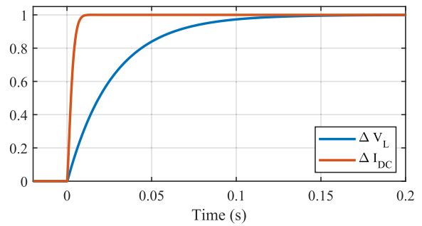
FIGURE 11. Dynamic response of the reference tracking of the inner and outer loop controllers.
