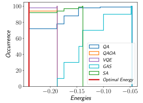
(c) Cumulative distribution of a Portfolio Optimization problem, where VQE emerges as better solver
