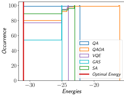
(a) Cumulative distribution of a Set Packing problem, where QA emerges as better solver
