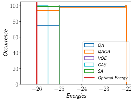
(d) Cumulative distribution of a Maxcut problem, where GAS emerges as better solver
