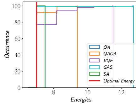
(e) Cumulative distribution of a Minimum Vertex Cover problem, where SA emerges as better solver
