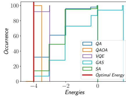
(b) Cumulative distribution of a Kclique problem, where QAOA emerges as better solver
