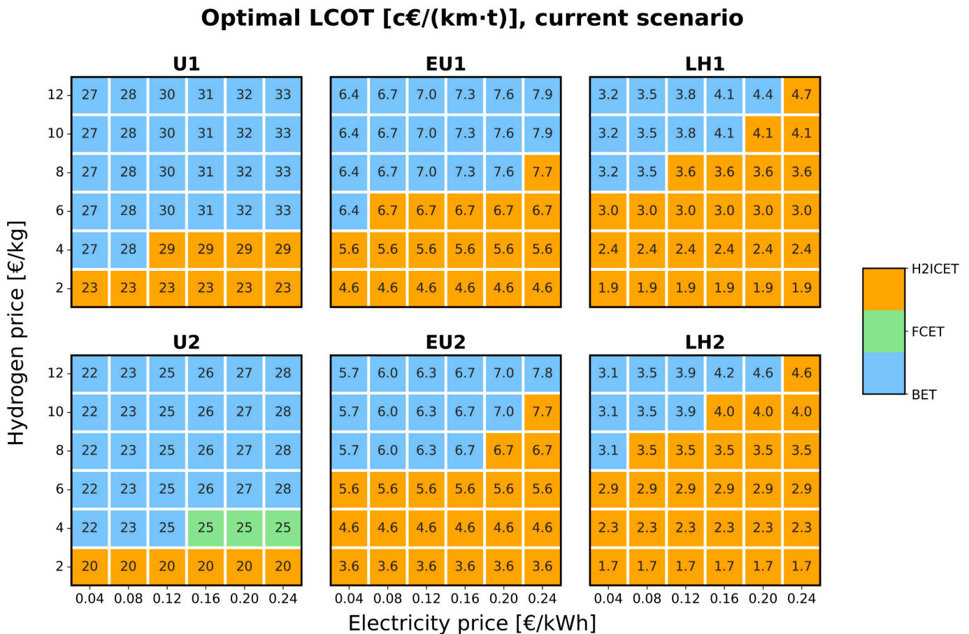
Fig. 7. Map of the cost-optimal solutions, in the current cost scenario, for the six investigated case studies under variable electricity (0.04–0.24 €/kWh) and hydrogen (2–12 €/kg) prices. The colour of the cell represents the cost-optimal powertrain among the three analysed.
