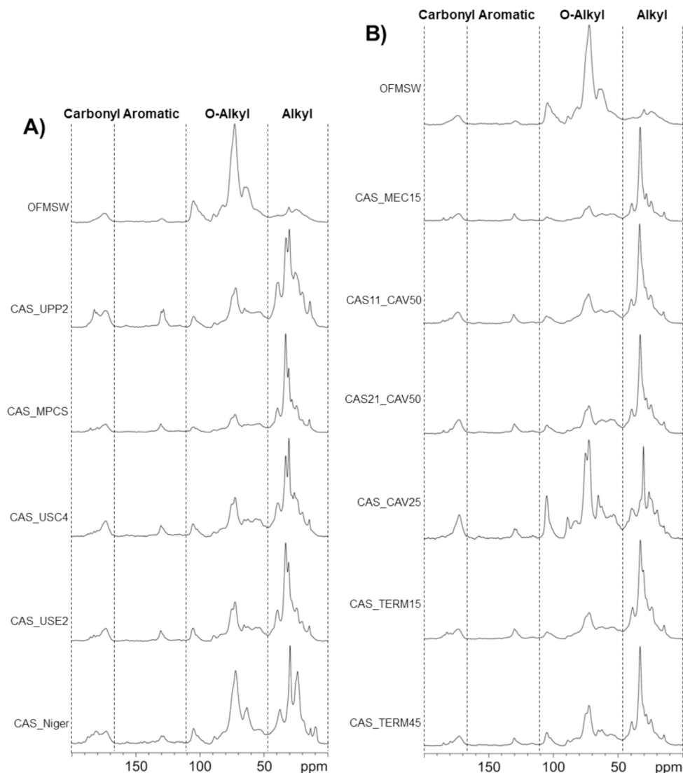
Fig. 4. Solid state ^{13}\text{C} NMR spectra of OFMSW and digestates from A) enzymatic pre-treatments and B) physical pre-treatments using CAS inoculum.
