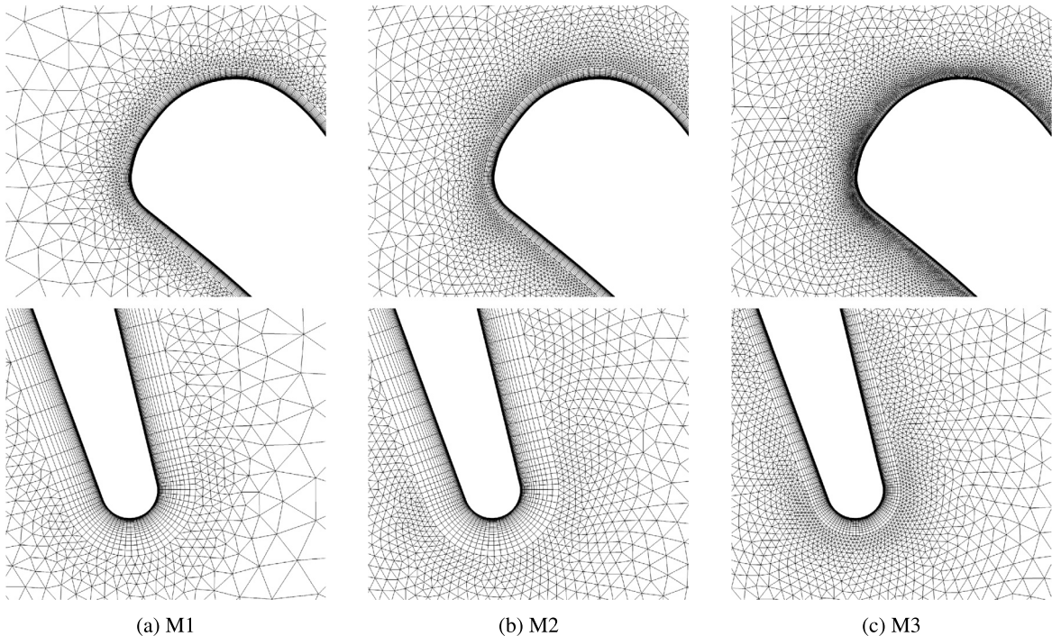
Fig. 12. LS89 - LE and TE mesh details.
