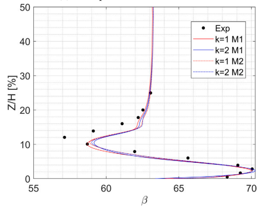
(b) Flow angle
