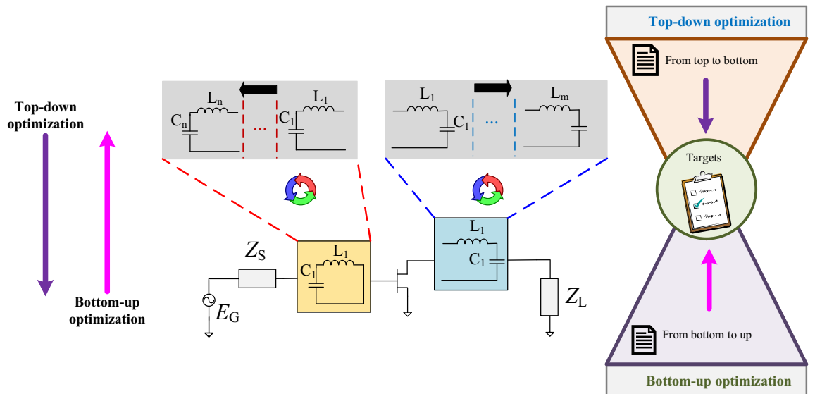
Figure 11. Illustration of BUO and TDO methods in configuring the initial structures of the amplifiers.
